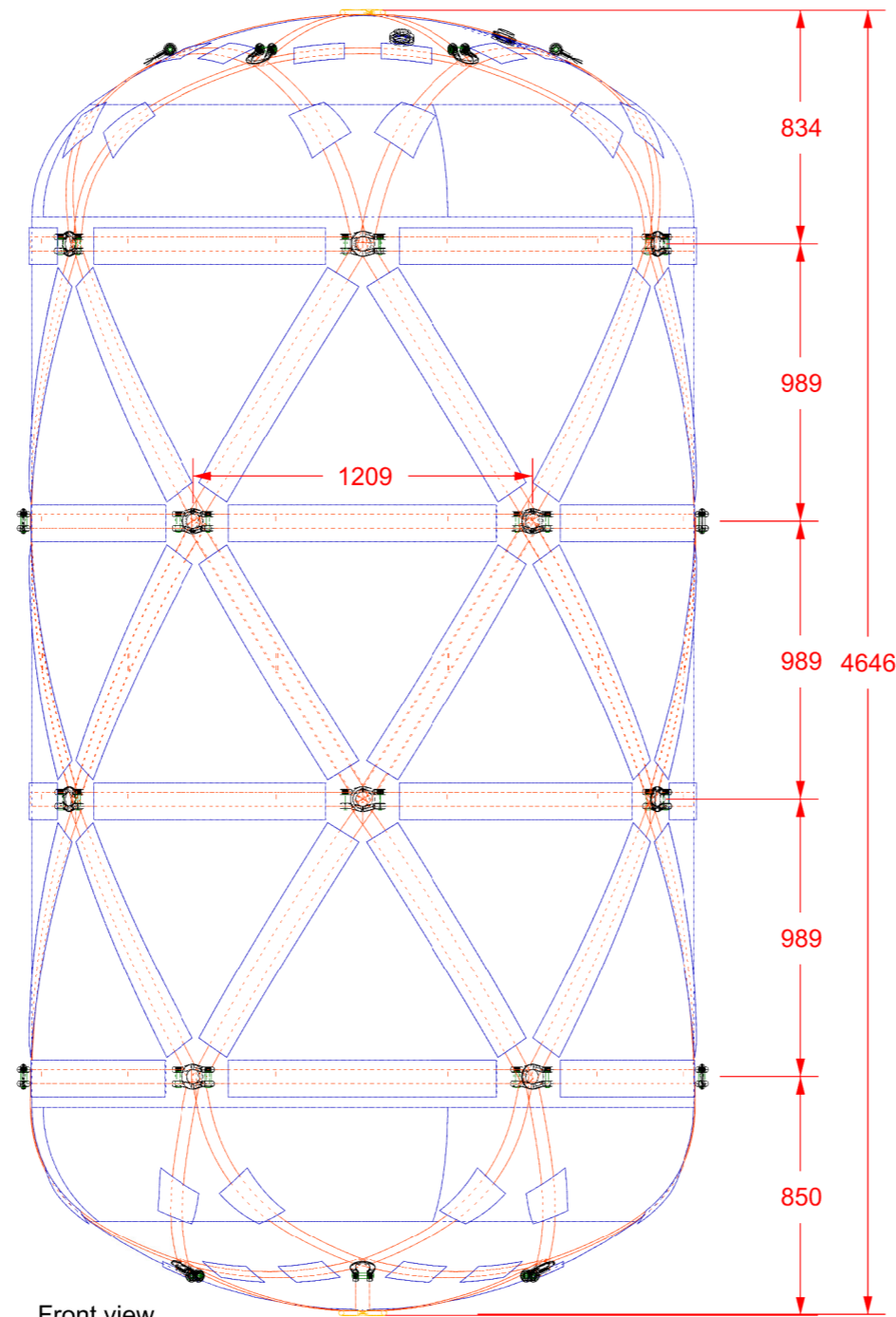
Front view
